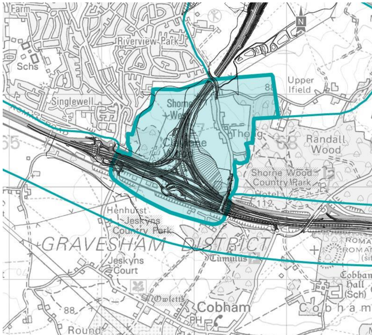
Plate 5.4 Section 2 – M2/A2/A122 Lower Thames Crossing junction
